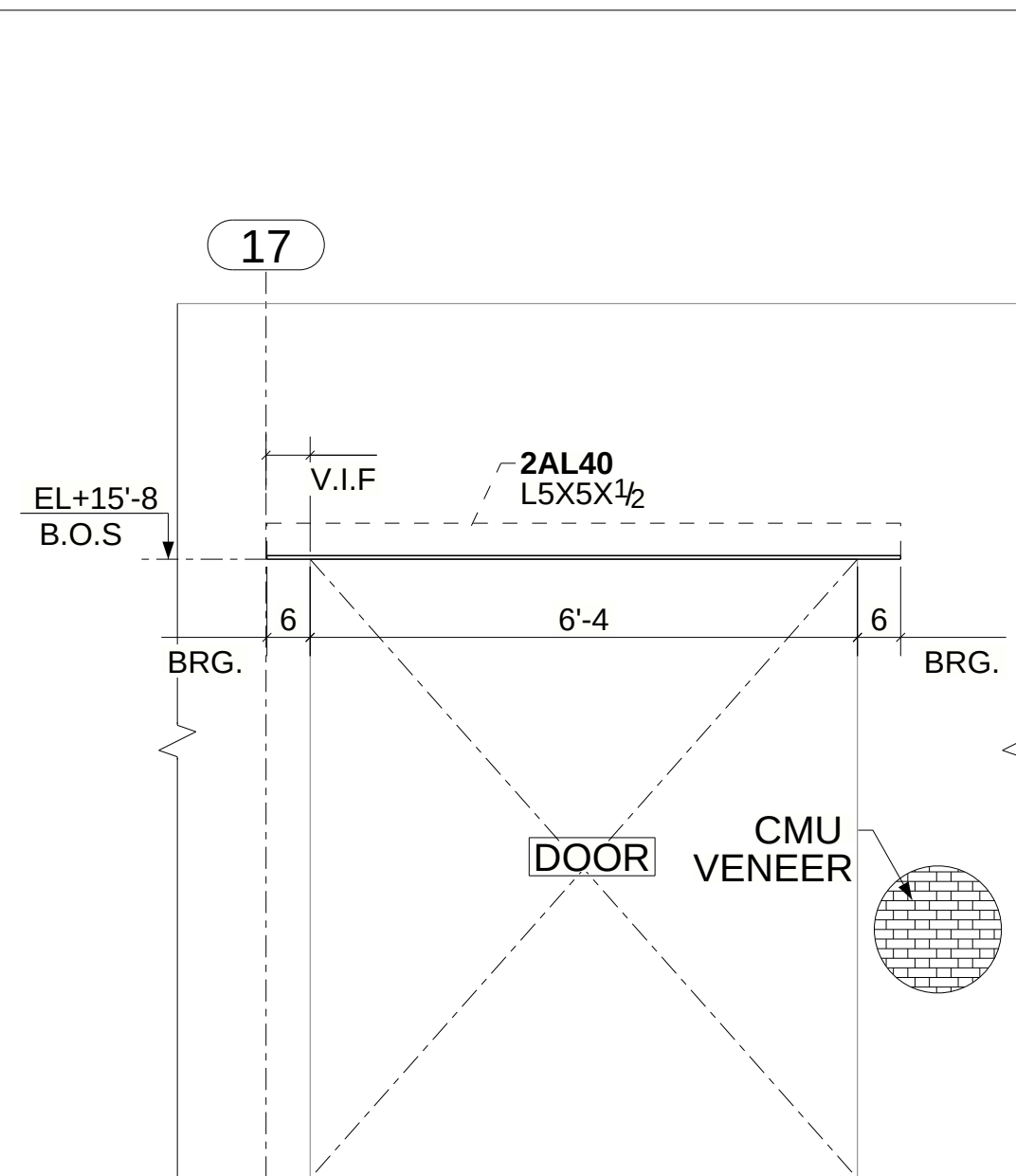
C - C (REF:1/A-201) (NORTH ELEVATION)
