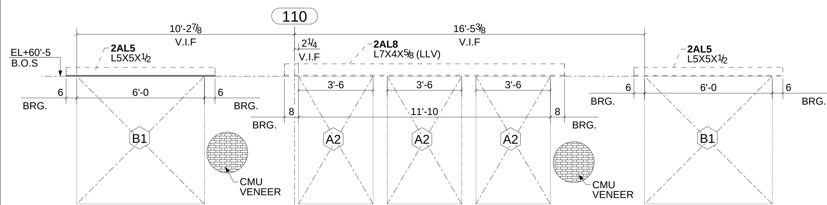
B - B (REF:1/A-201) (NORTH ELEVATION)
