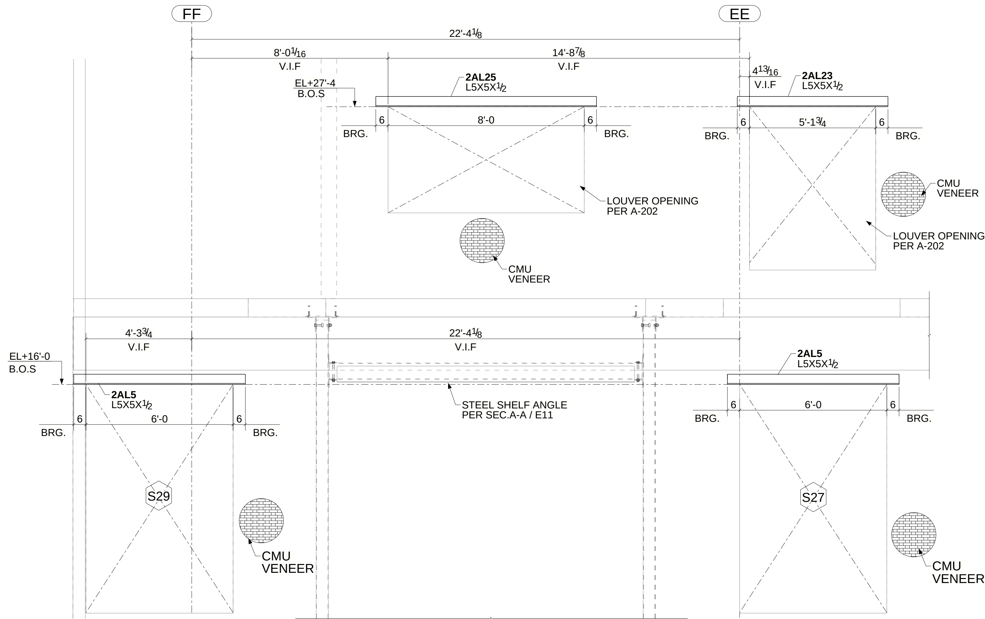
D - D (REF:1/A-202) (WEST ELEVATION)
