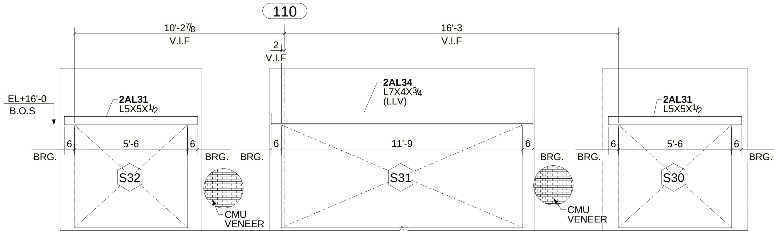
A - A (REF:1/A-201) (NORTH ELEVATION)
