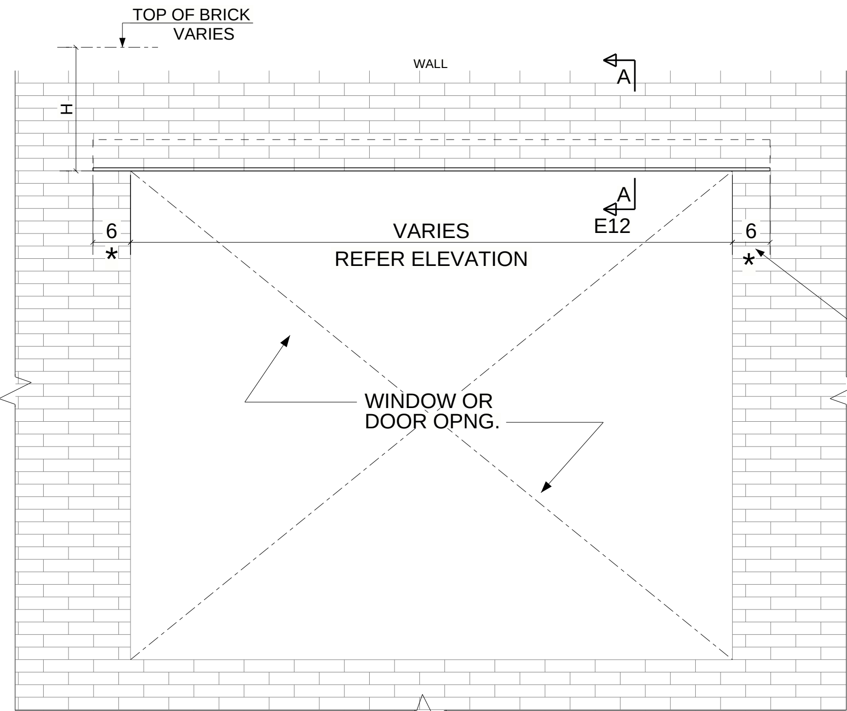
TYPICAL STEEL ANGLE BRICK LOOSE LINTEL ELEVATION DETAIL AT WINDOWS, DOORS AND STORE FRONTS. (REF: 12/S-421)
